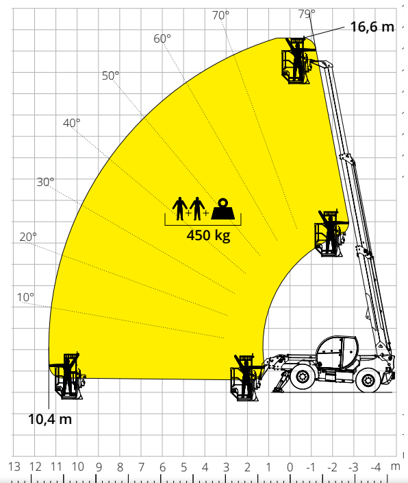
Load chart with PLATFORM, 450 kg, FOR MINES ATT - 01 - 027
